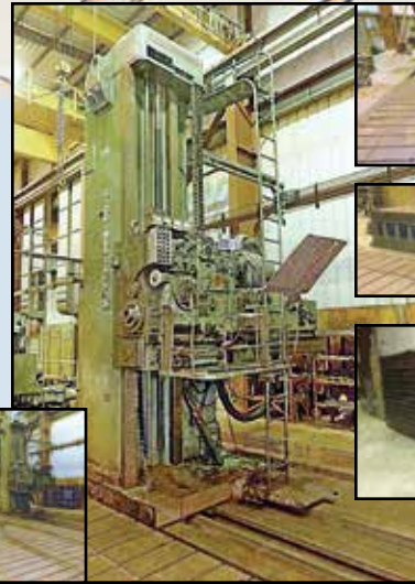
GIDDINGS & LEWIS 570 Four Horizontal Boring Mill , 7" spindle, #7 Morse taper, X=432", Y=192", Z=156" vertical, 44" runway, w/Trak i02 2-axis DRO, SN 280-1455.
