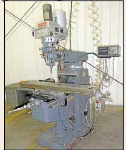
ACRA Vertical Mill , Mdl. CK 1-1/2 HK, 10" x 54" table, VS, 3 HP, power draw bar, PF@X, w/Mitutoyo 2-axis DRO, SN 771407.
