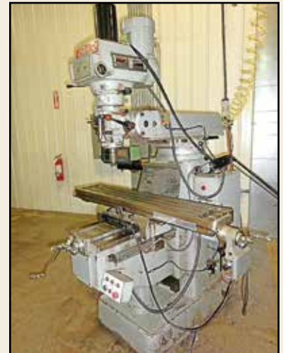
CAMTROL, INC. Vertical Mill , 10" x 50" table, power draw bar, PF@X, w/Mitutoyo 2-axis DRO, SN N/A.
