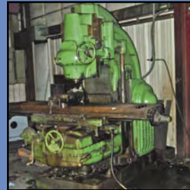
MILWAUKEE Mdl. K 18" x 83" Vertical Mill, table, 6" machine vise, s/n 17-4233.
